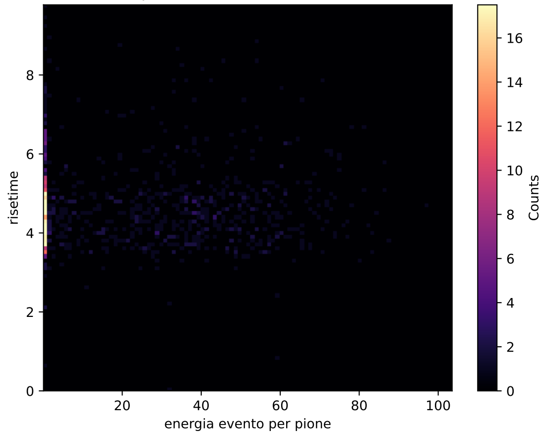
pion distribution 100.0GeV
