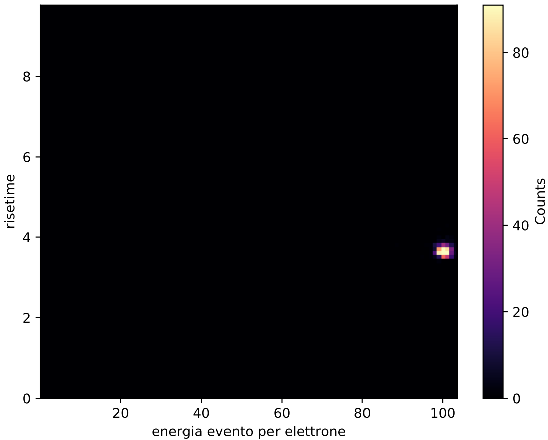
electron distribution 100.0GeV
